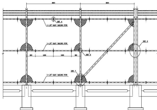
FENCE ELEVATION SC 1:20
